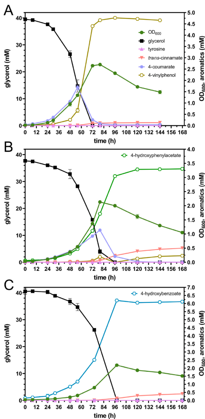
Fig. 5. Shake flask cultivations of GRC3Δ5-TYR3 with integrated expression cassette of either attTn7::Kan_FRT_P14f-RtPAL-pdc (A), attTn7::Kan_FRT_P14f-RtPAL-pdc-styABC (B), or attTn7::Kan_FRT_P14f-RtPAL-ech-vdh-fcs (C) cultivated in MSM with 40 mM glycerol. The medium was one-fold-buffered for production of 4-vinylphenol and two-fold-buffered for production of 4-hydroxyphenylacetate and 4-hydroxybenzoate. Error bars indicate the standard deviation of replicates (n = 3).
