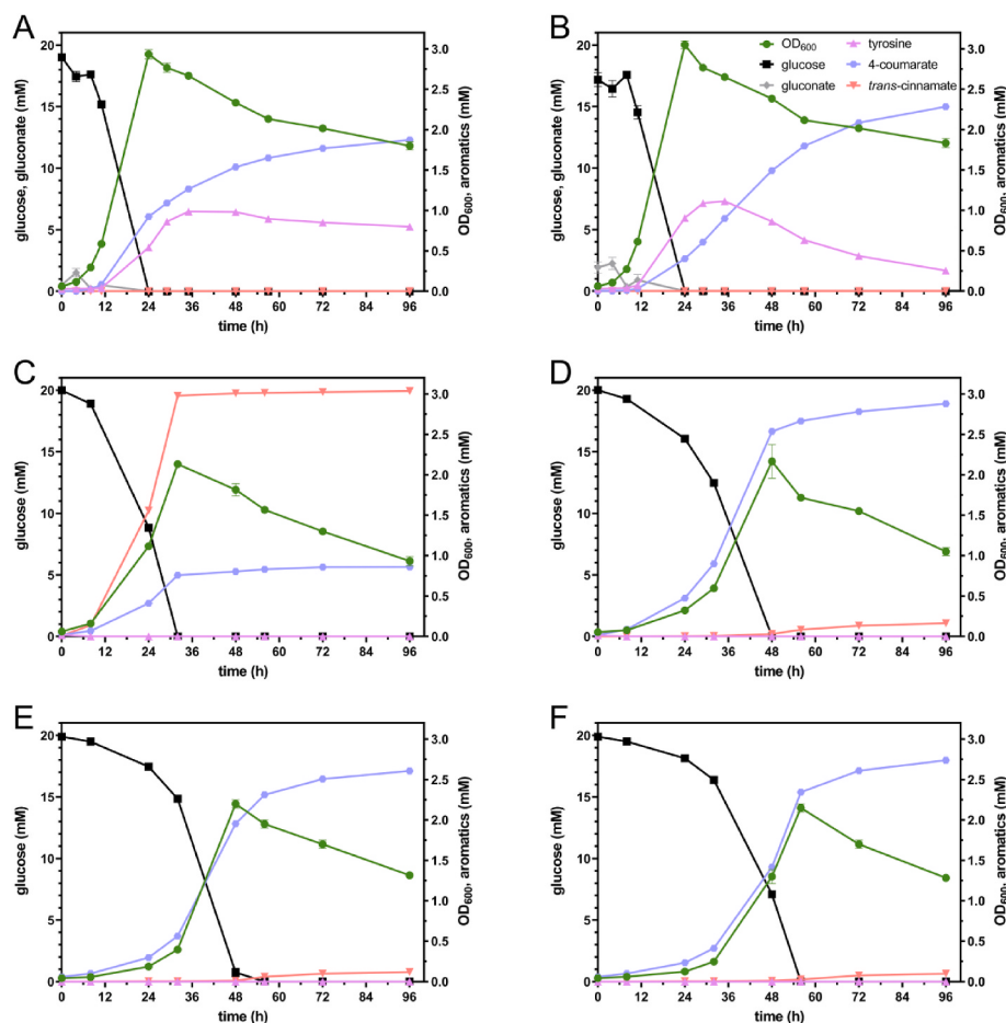
Fig. 3. Shake flask cultivations of selected strains for the production of 4-coumarate: GRC3Δ5-TYR2 with pJNNopt- FjTAL (A), pJNNopt- StsTAL (B), or pJNNopt- RtPAL (C), GRC3Δ5-TYR3 with pJNNopt- RtPAL (D), GRC3Δ5-TYR3- attTn7::P 14f -RtPAL (E), and GRC3Δ5-TYR4.1- attTn7::P 14f -RtPAL (F) in MSM (two-fold-buffered) with 20 mM glucose. Error bars indicate the standard deviation of replicates ( n = 3 ).
