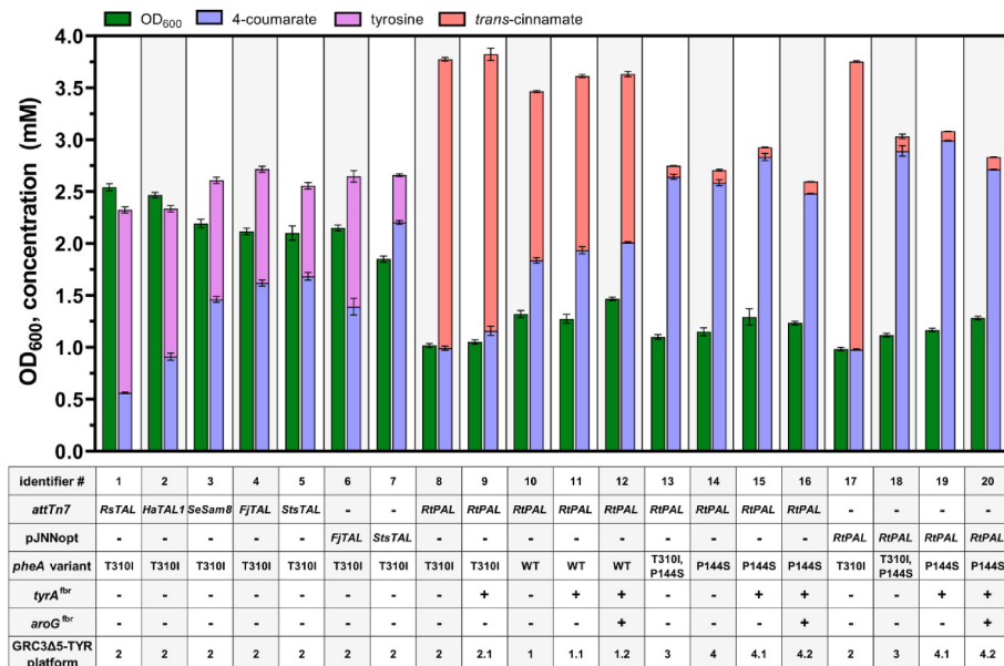
Fig. 2. 4-Coumarate production using ammonia-lyases from R. sphaeroides (RsTAL), H. aurantiacus (HaTAL1), S. espanaensis (SeSam8), F. johnsoniae (FjTAL), Streptomyces sp. (StsTAL), and R. toruloides (RtPAL). PAL/TAL genes were either chromosomally ( attTn7 ) or episomally (pJNNOpt) expressed in tyrosine-overproducing P. taiwanensis GRC3Δ5-TYR2. RtPAL was also assessed in combination with different pheA genotypes and/or heterologous expression of tyrA tr and aroG tr that were integrated into the chromosome under the control of synthetic promoter P 14e . Strains were grown in 24-well microtiter plates using mineral salt medium (MSM, three-fold-buffered) with 20 mM glucose as sole carbon source for 96 h to ensure glucose depletion. Error bars indicate the standard deviation of biological replicates. For selected strains, the cultivation experiment was performed multiple times ( n \geq 3 ).
