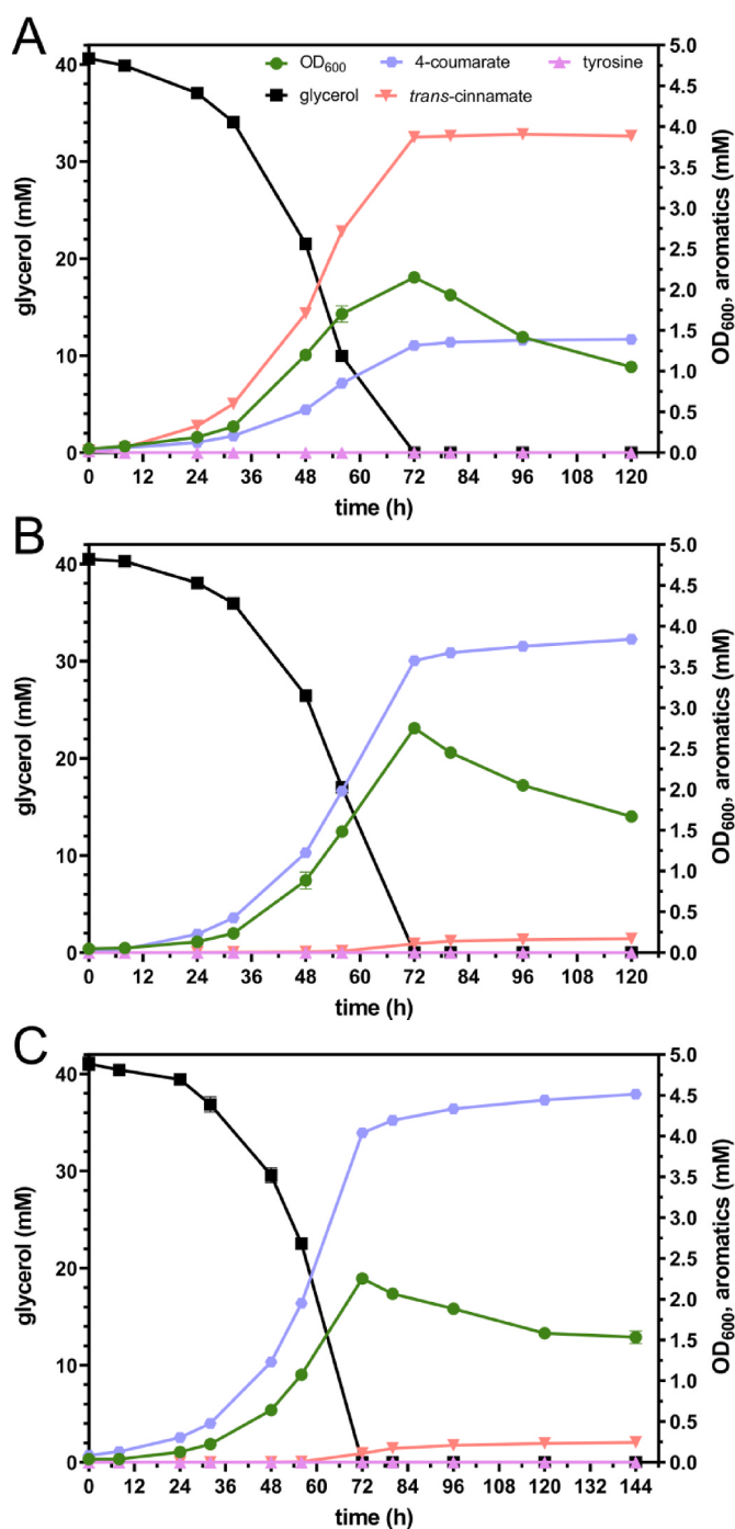
Fig. 4. Shake flask cultivations of GRC3Δ5-TYR2 pJNNopt-RtPAL (A), GRC3Δ5-TYR3 pJNNopt-RtPAL (B), and GRC3Δ5-TYR3-attTn7::P14f-RtPAL (C) in MSM (two-fold-buffered) with 40 mM glycerol. Error bars indicate the standard deviation of replicates (n = 3).
